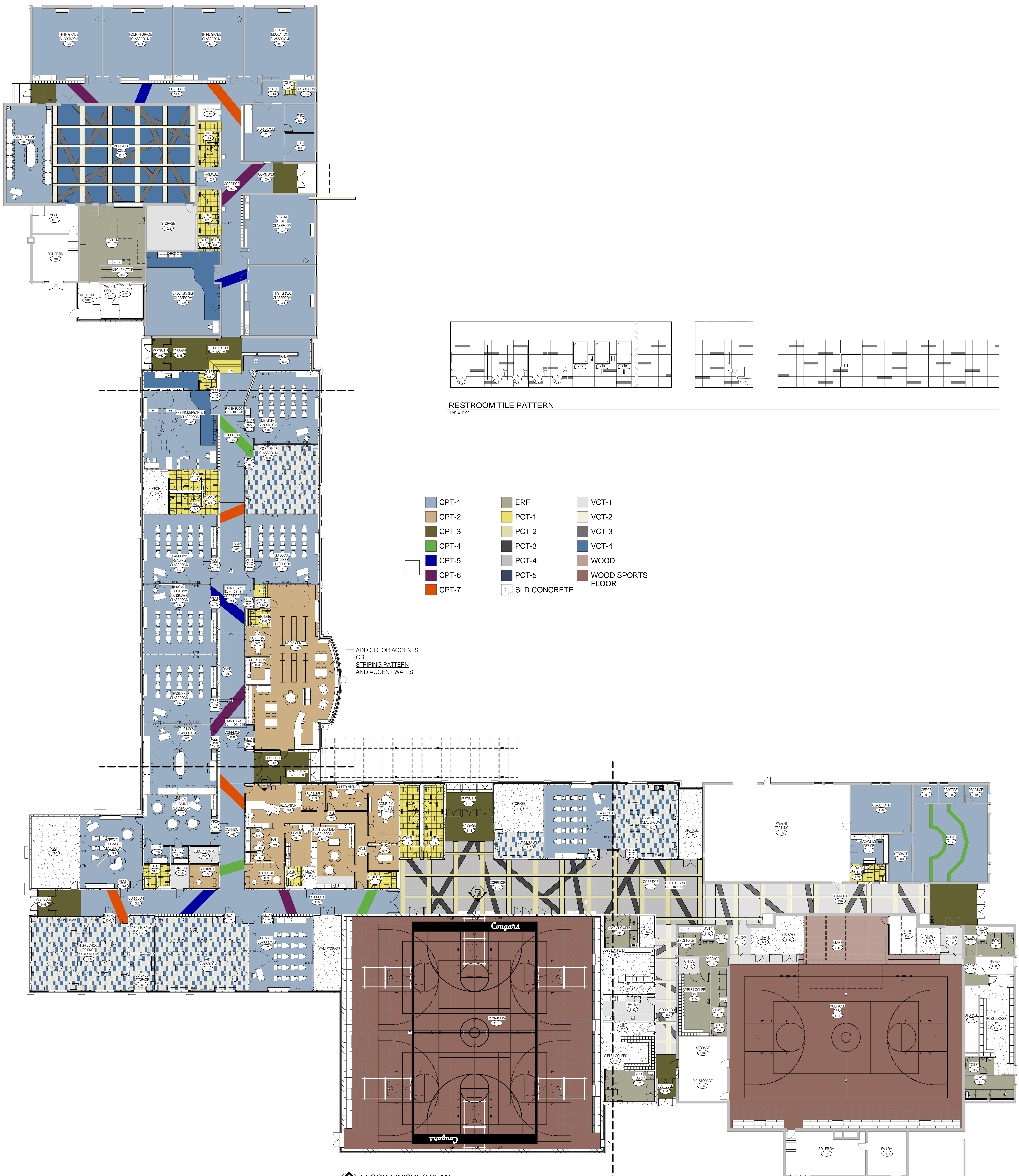
FLOOR FINISHES PLAN 1:145
